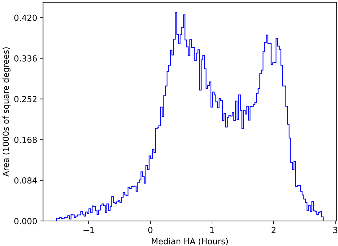
too_elab_r64_d3_giz_v3.4_10yrs All sky z band: Median HA
