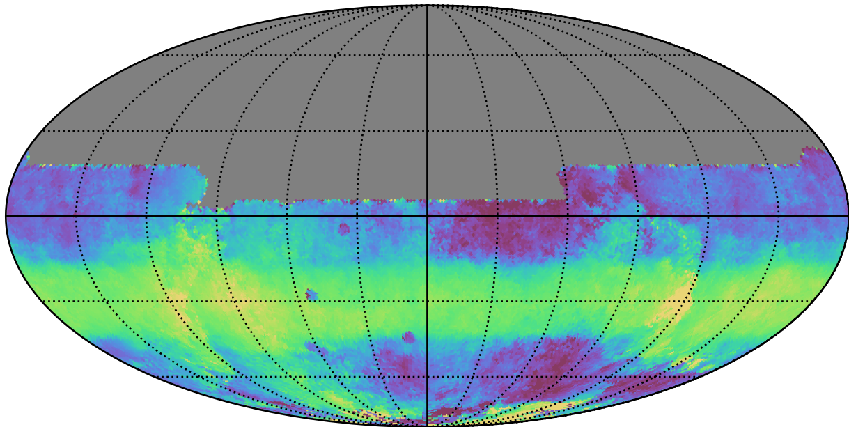
too_elab_r64_d3_giz_v3.4_10yrs All sky y band: Median HA
