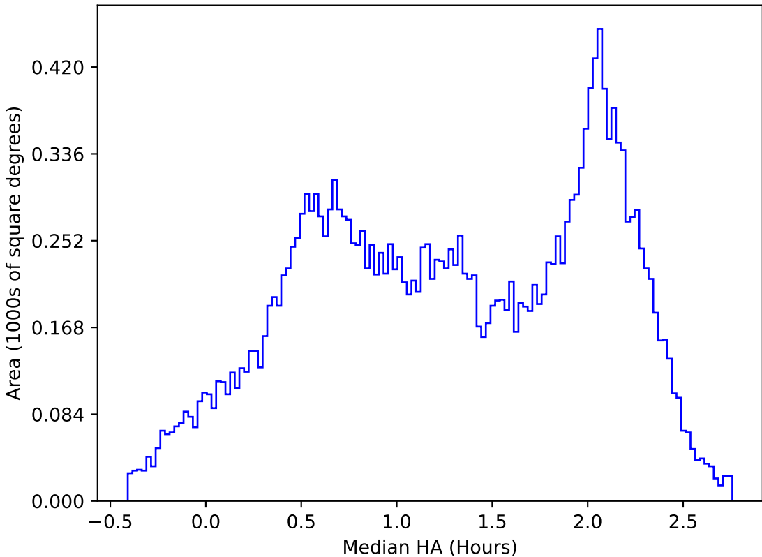
too_elab_r64_d3_giz_v3.4_10yrs All sky y band: Median HA
