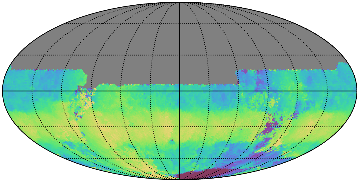
too_elab_r64_d3_giz_v3.4_10yrs All sky u band: Median HA
