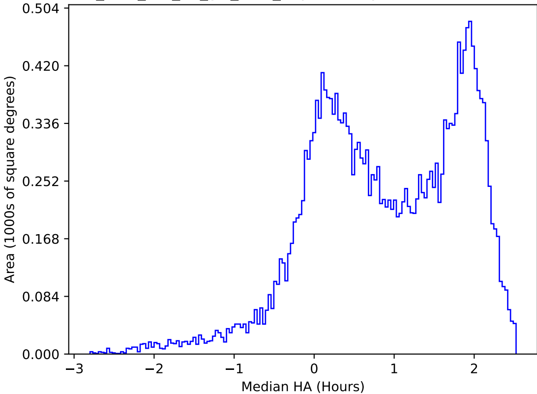
too_elab_r64_d3_giz_v3.4_10yrs All sky u band: Median HA
