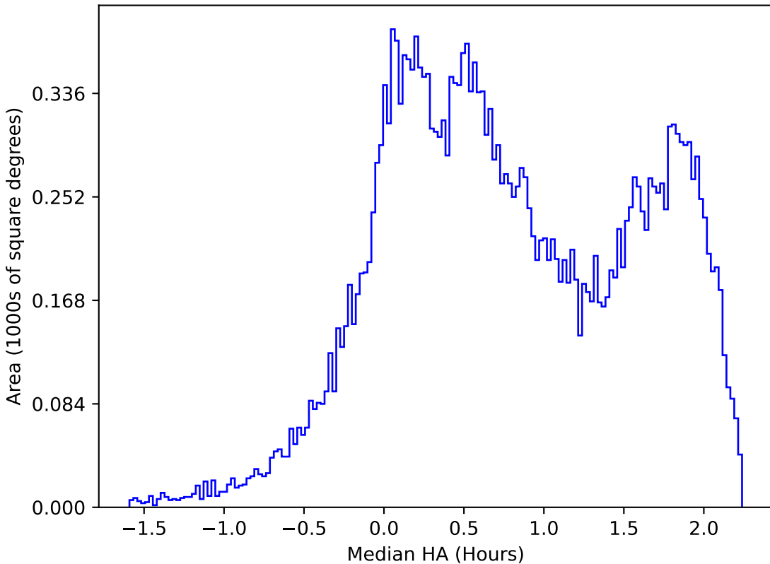
too_elab_r64_d3_giz_v3.4_10yrs All sky r band: Median HA
