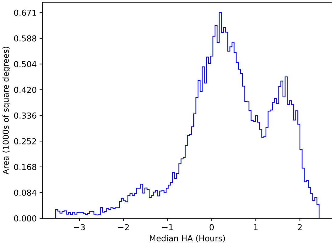
too_elab_r64_d3_giz_v3.4_10yrs All sky g band: Median HA
