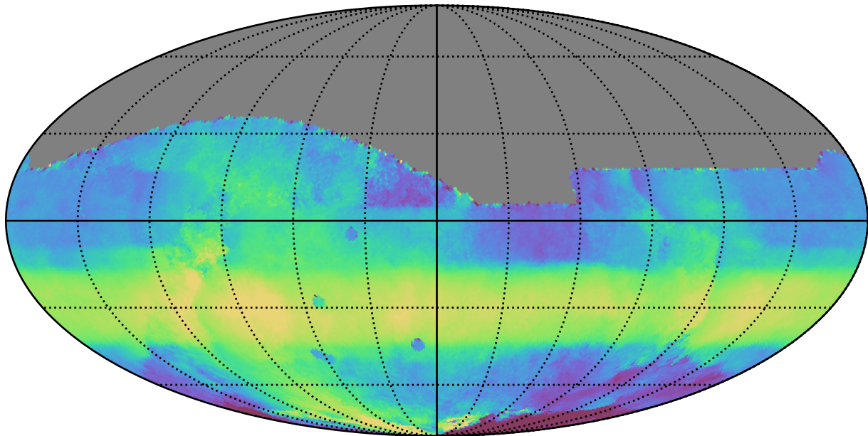
too_elab_r64_d3_giz_v3.4_10yrs All sky all bands: Median HA
