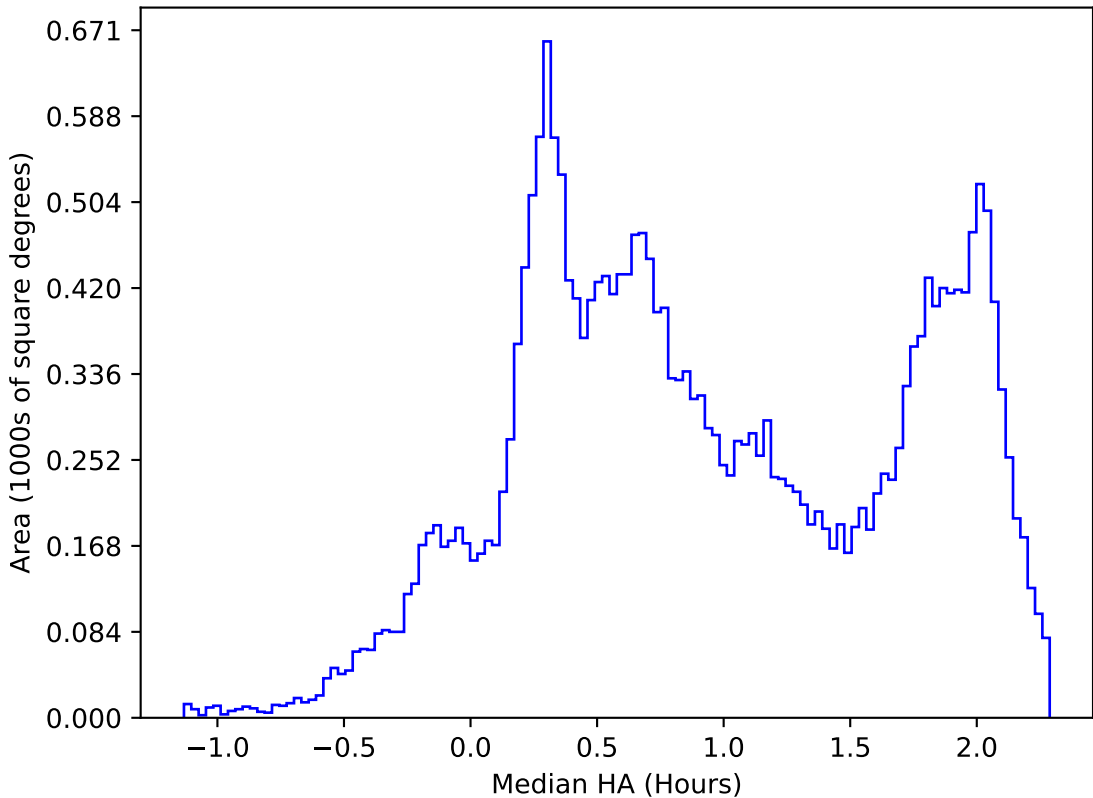
too_elab_r64_d3_giz_v3.4_10yrs All sky all bands: Median HA
