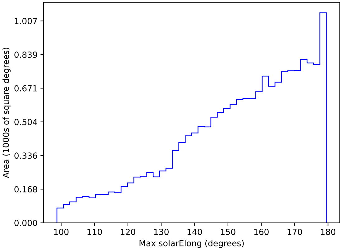
too_elab_r64_d3_giz_v3.4_10yrs WFD z band: Max solarElong
