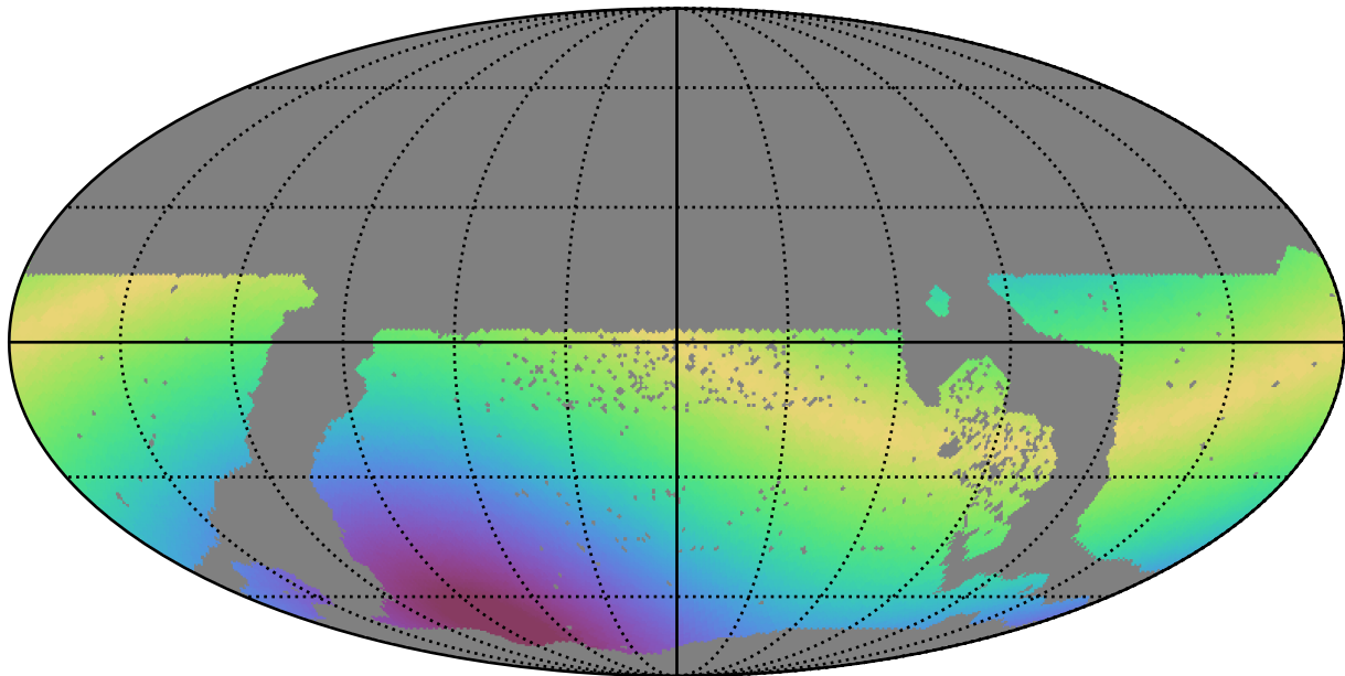
too_elab_r64_d3_giz_v3.4_10yrs WFD y band: Max solarElong
