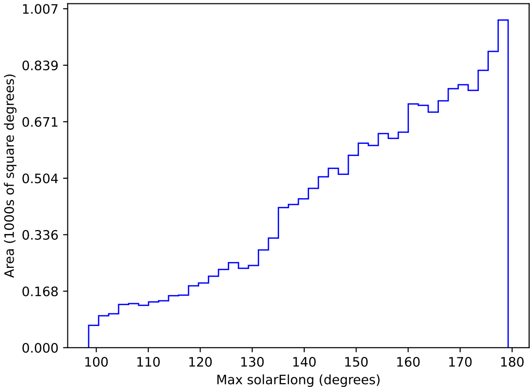
too_elab_r64_d3_giz_v3.4_10yrs WFD y band: Max solarElong
