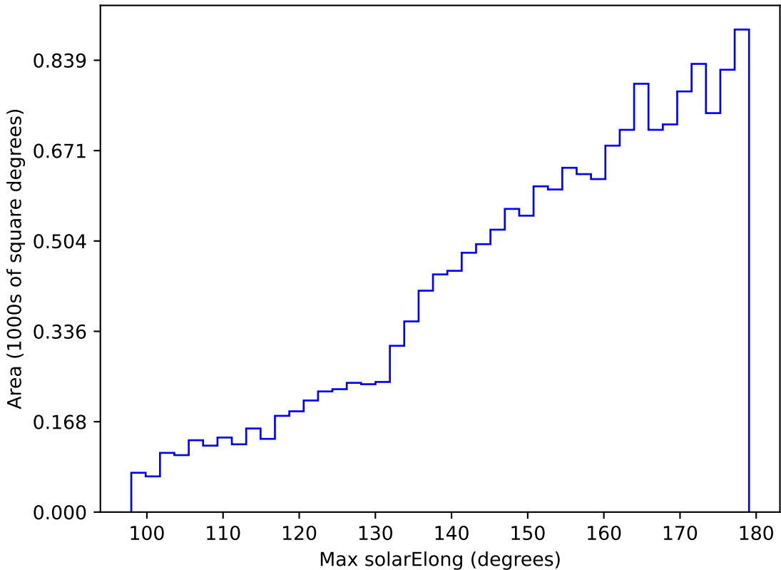
too_elab_r64_d3_giz_v3.4_10yrs WFD u band: Max solarElong
