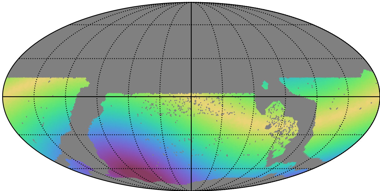
too_elab_r64_d3_giz_v3.4_10yrs WFD i band: Max solarElong
