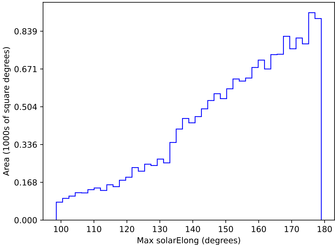
too_elab_r64_d3_giz_v3.4_10yrs WFD g band: Max solarElong
