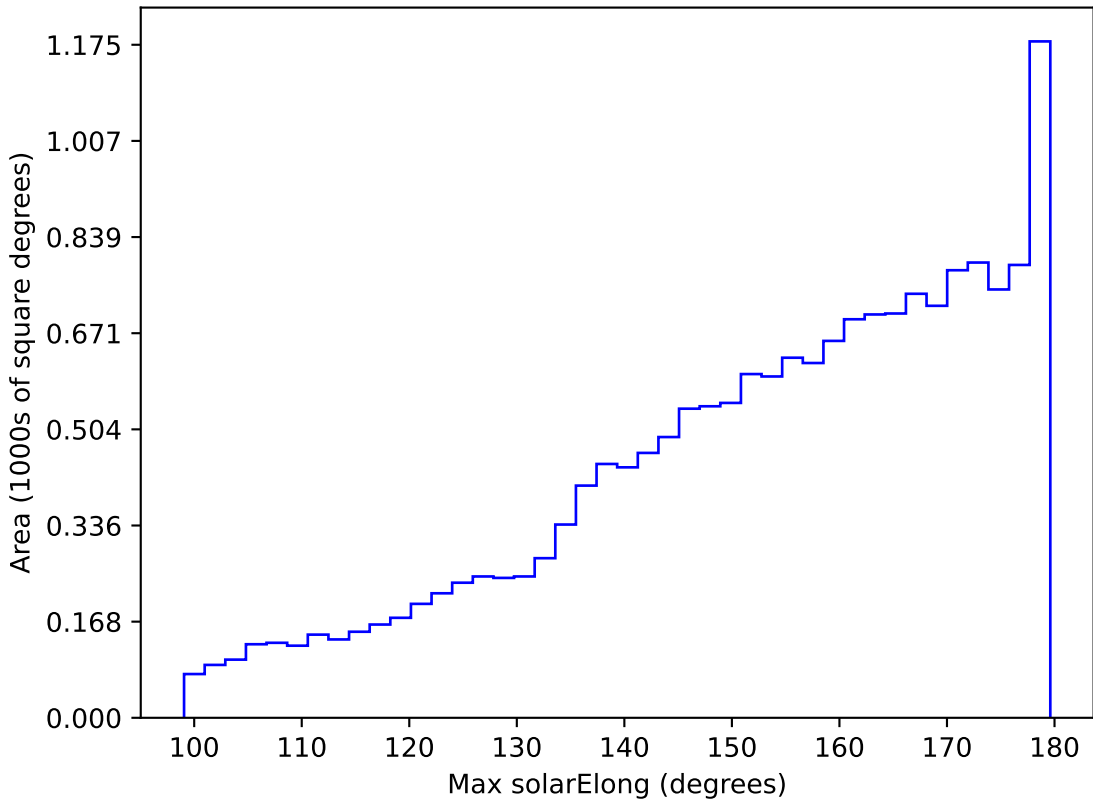
too_elab_r64_d3_giz_v3.4_10yrs WFD all bands: Max solarElong
