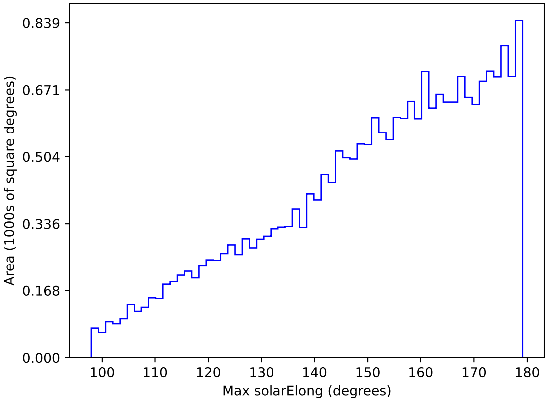
too_elab_r64_d3_giz_v3.4_10yrs All sky y band: Max solarElong
