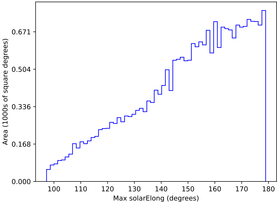
too_elab_r64_d3_giz_v3.4_10yrs All sky u band: Max solarElong
