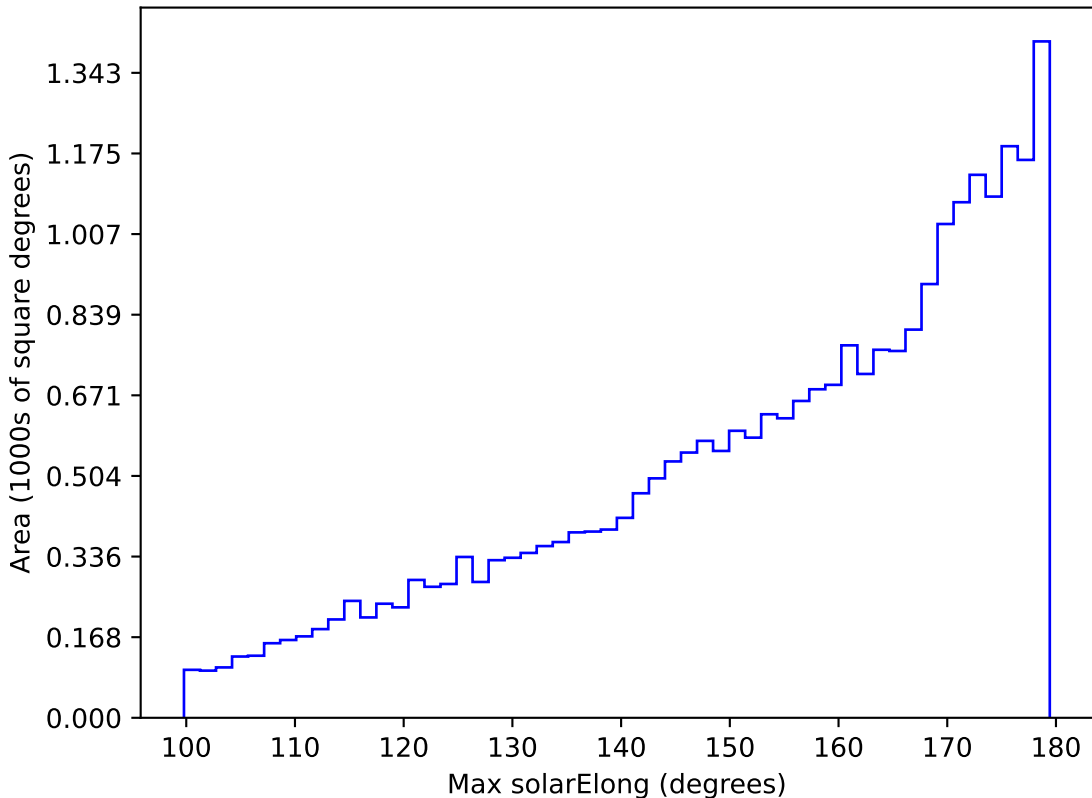
too_elab_r64_d3_giz_v3.4_10yrs All sky i band: Max solarElong
