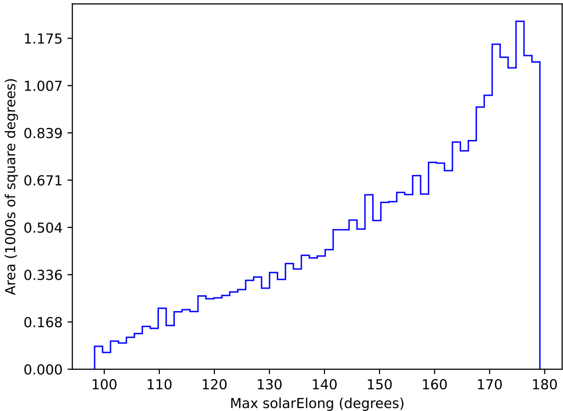
too_elab_r64_d3_giz_v3.4_10yrs All sky g band: Max solarElong
