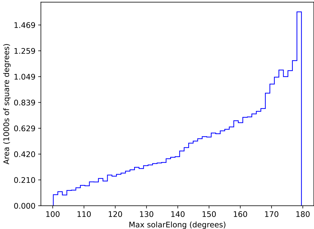
too_elab_r64_d3_giz_v3.4_10yrs All sky all bands: Max solarElong
