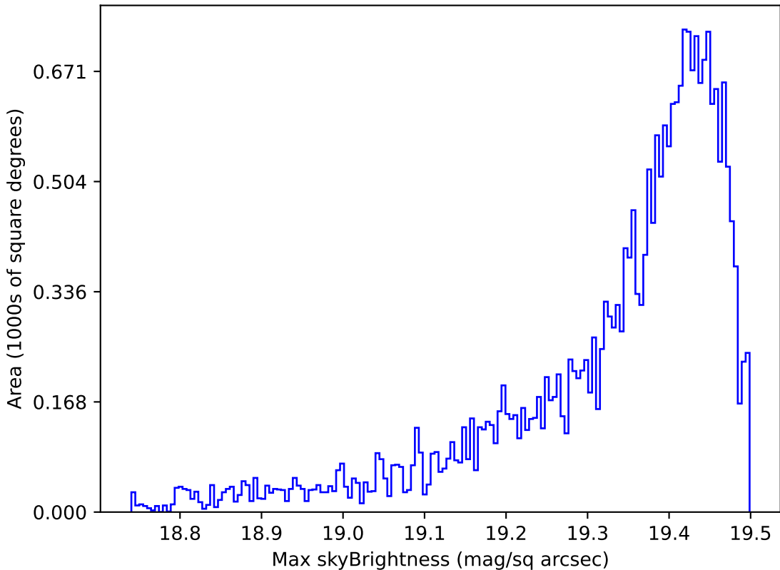
too_elab_r64_d3_giz_v3.4_10yrs Yr 1 z band: Max skyBrightness
