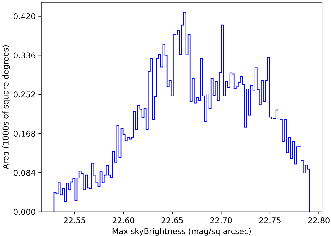
too_elab_r64_d3_giz_v3.4_10yrs Yr 1 u band: Max skyBrightness
