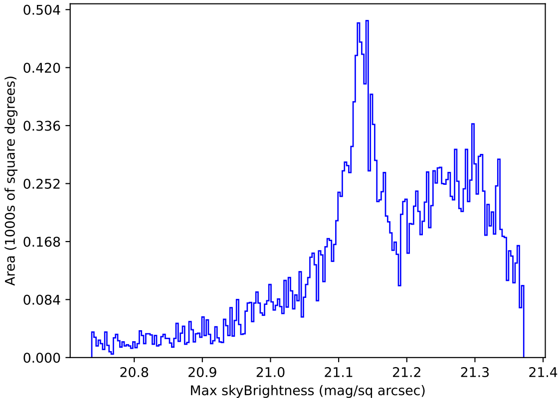
too_elab_r64_d3_giz_v3.4_10yrs Yr 1 r band: Max skyBrightness
