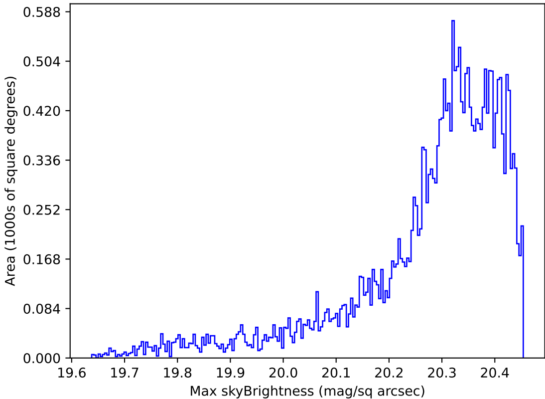
too_elab_r64_d3_giz_v3.4_10yrs Yr 1 i band: Max skyBrightness
