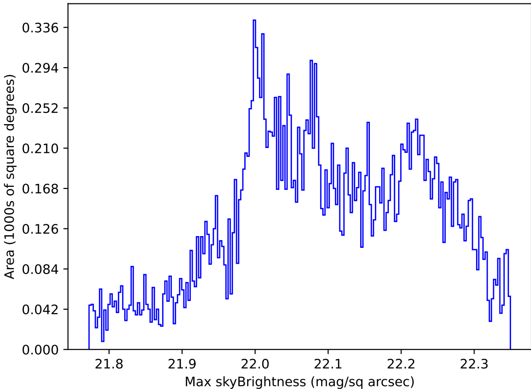
too_elab_r64_d3_giz_v3.4_10yrs Yr 1 g band: Max skyBrightness
