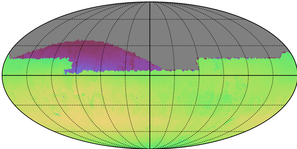
too_elab_r64_d3_giz_v3.4_10yrs Yr 1 all bands: Max skyBrightness
