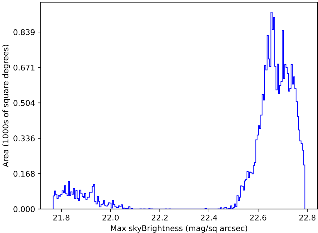
too_elab_r64_d3_giz_v3.4_10yrs Yr 1 all bands: Max skyBrightness
