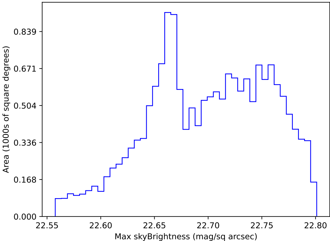
too_elab_r64_d3_giz_v3.4_10yrs WFD u band: Max skyBrightness
