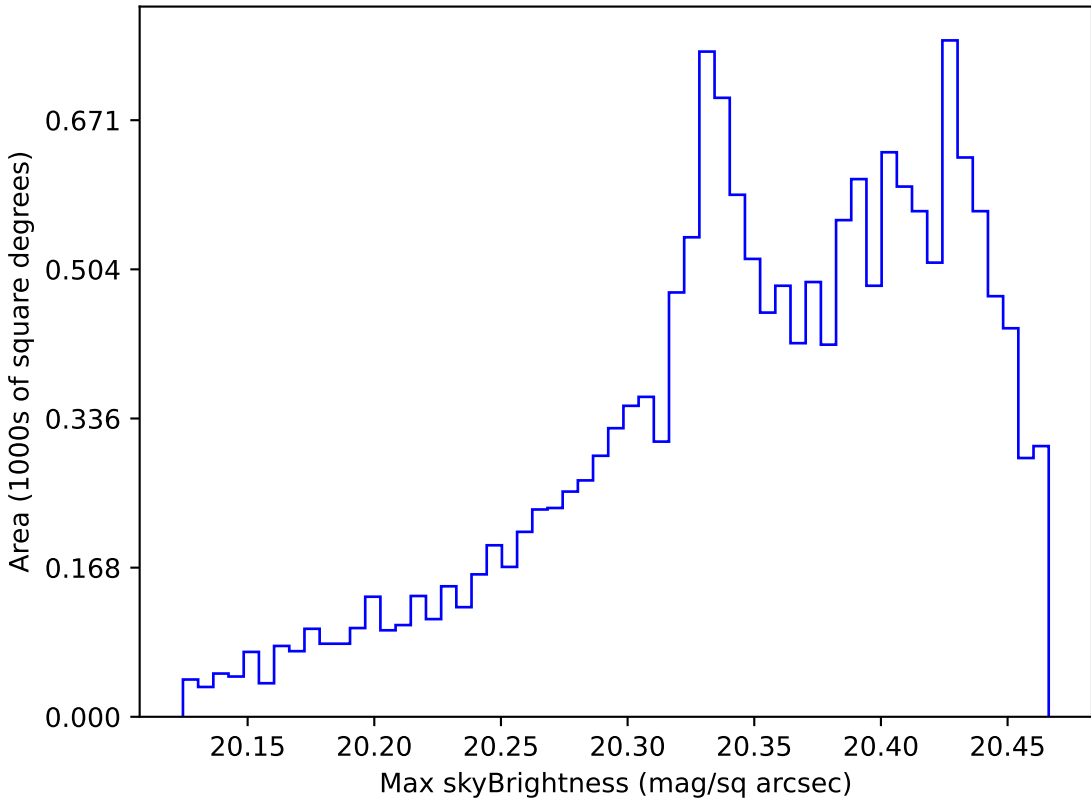
too_elab_r64_d3_giz_v3.4_10yrs WFD i band: Max skyBrightness
