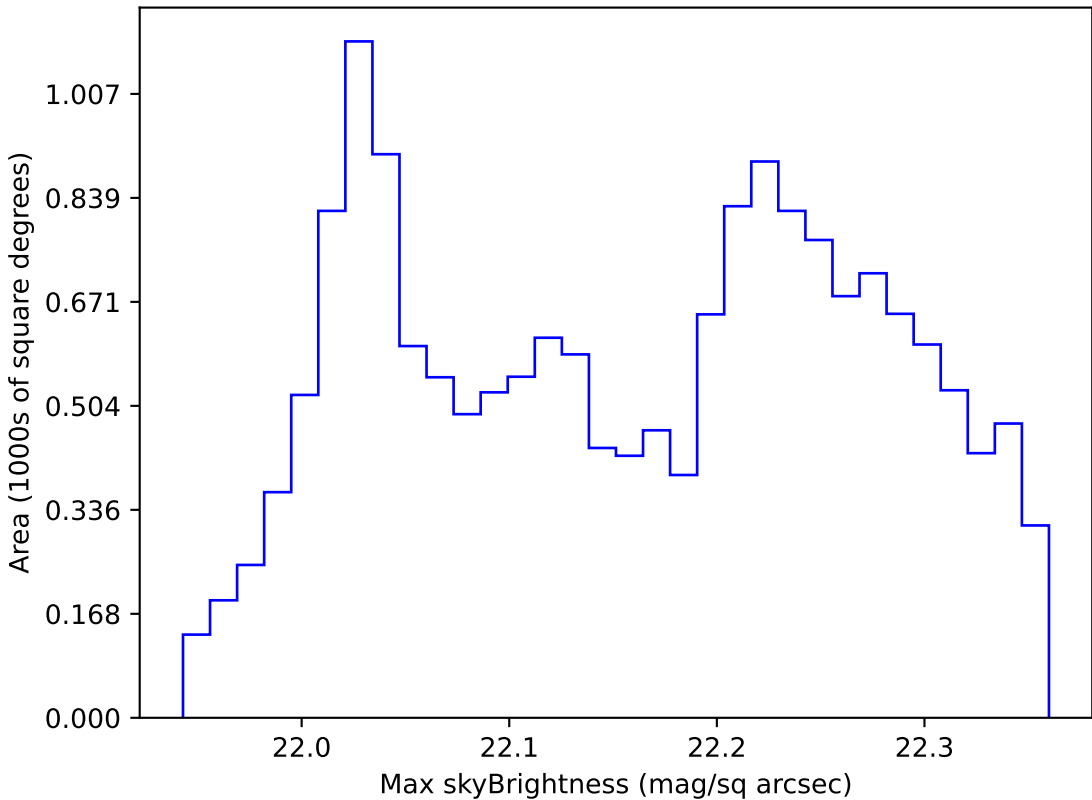
too_elab_r64_d3_giz_v3.4_10yrs WFD g band: Max skyBrightness
