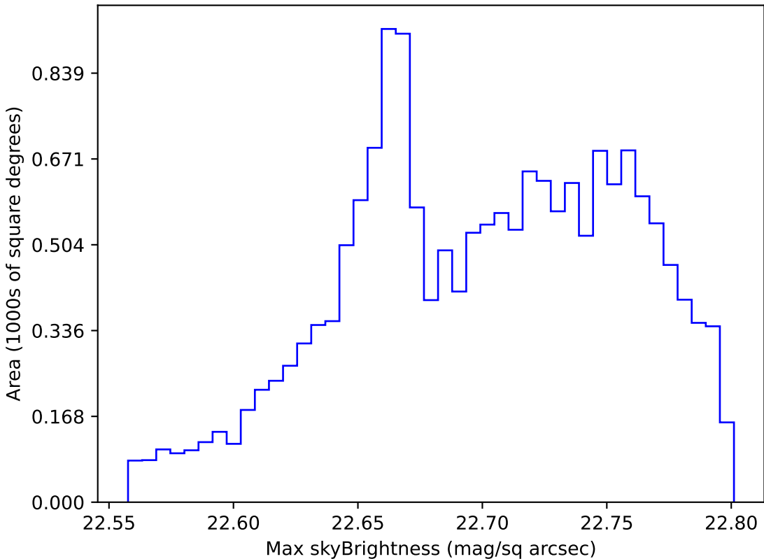
too_elab_r64_d3_giz_v3.4_10yrs WFD all bands: Max skyBrightness
