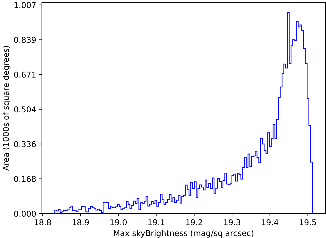
too_elab_r64_d3_giz_v3.4_10yrs All sky z band: Max skyBrightness
