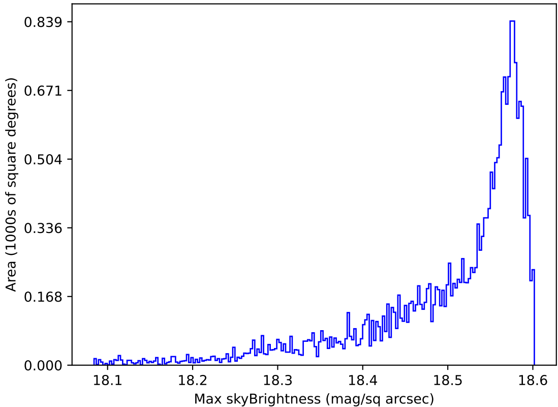
too_elab_r64_d3_giz_v3.4_10yrs All sky y band: Max skyBrightness
