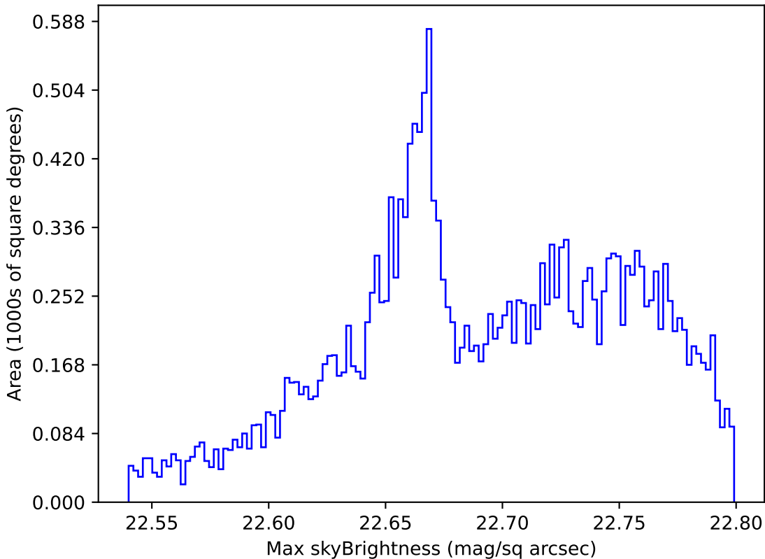
too_elab_r64_d3_giz_v3.4_10yrs All sky u band: Max skyBrightness
