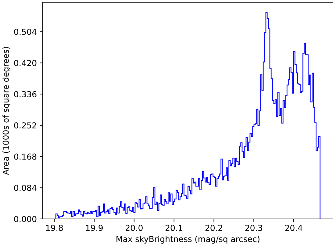
too_elab_r64_d3_giz_v3.4_10yrs All sky i band: Max skyBrightness
