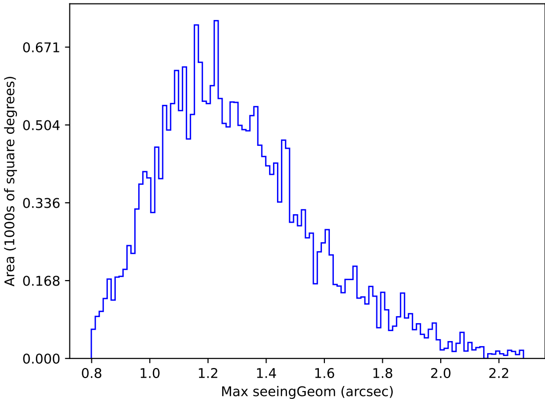
too_elab_r64_d3_giz_v3.4_10yrs Yr 1 z band: Max seeingGeom
