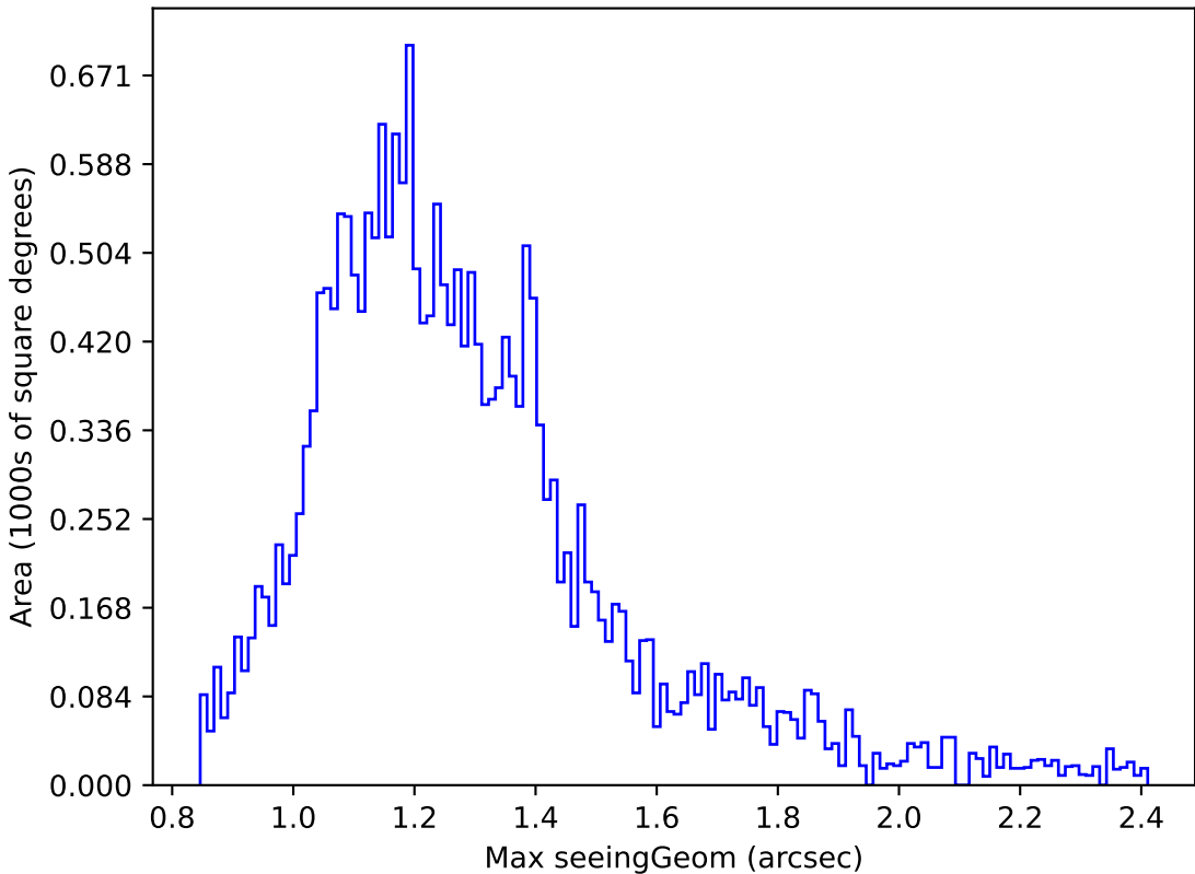
too_elab_r64_d3_giz_v3.4_10yrs Yr 1 y band: Max seeingGeom
