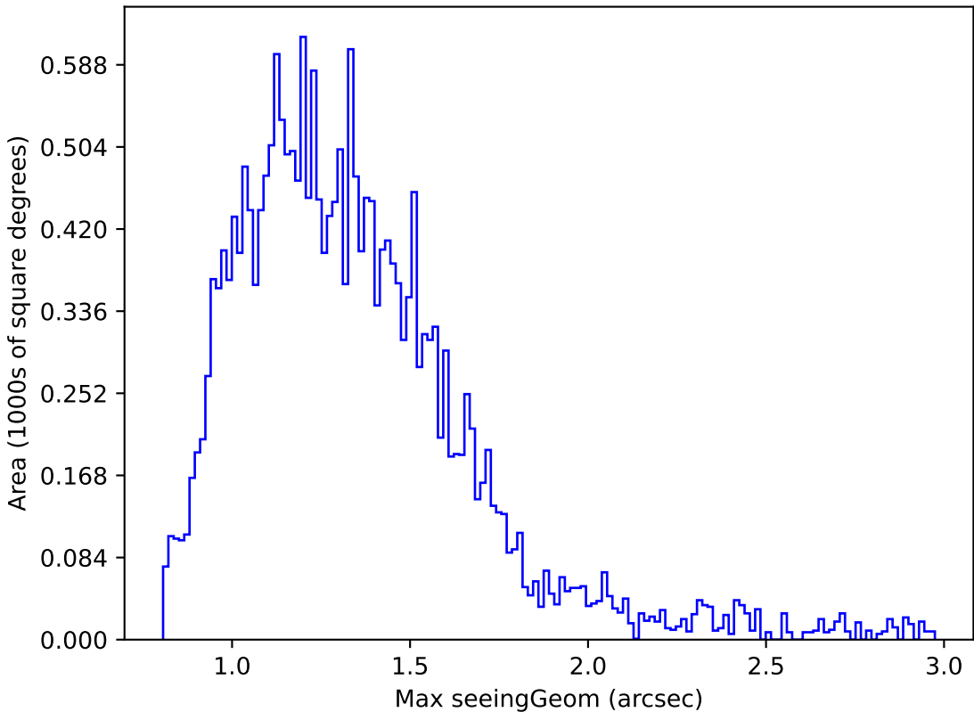
too_elab_r64_d3_giz_v3.4_10yrs Yr 1 u band: Max seeingGeom
