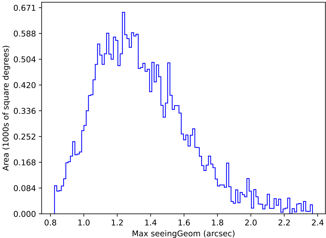
too_elab_r64_d3_giz_v3.4_10yrs Yr 1 r band: Max seeingGeom
