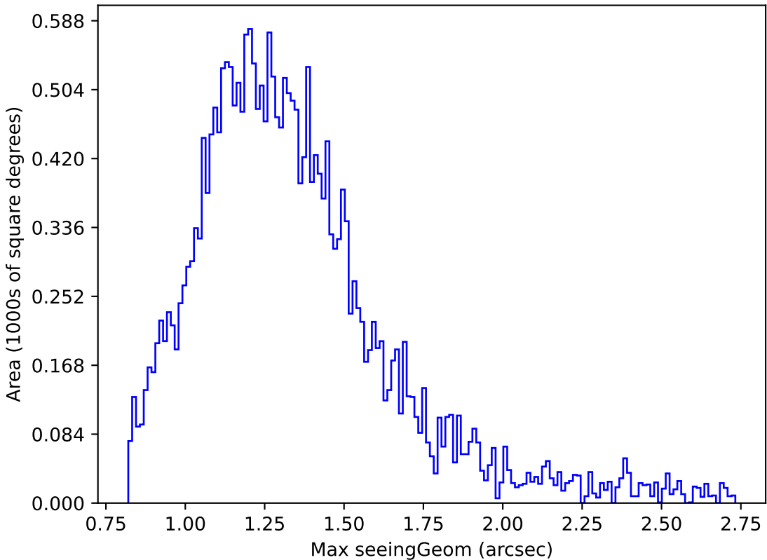
too_elab_r64_d3_giz_v3.4_10yrs Yr 1 i band: Max seeingGeom
