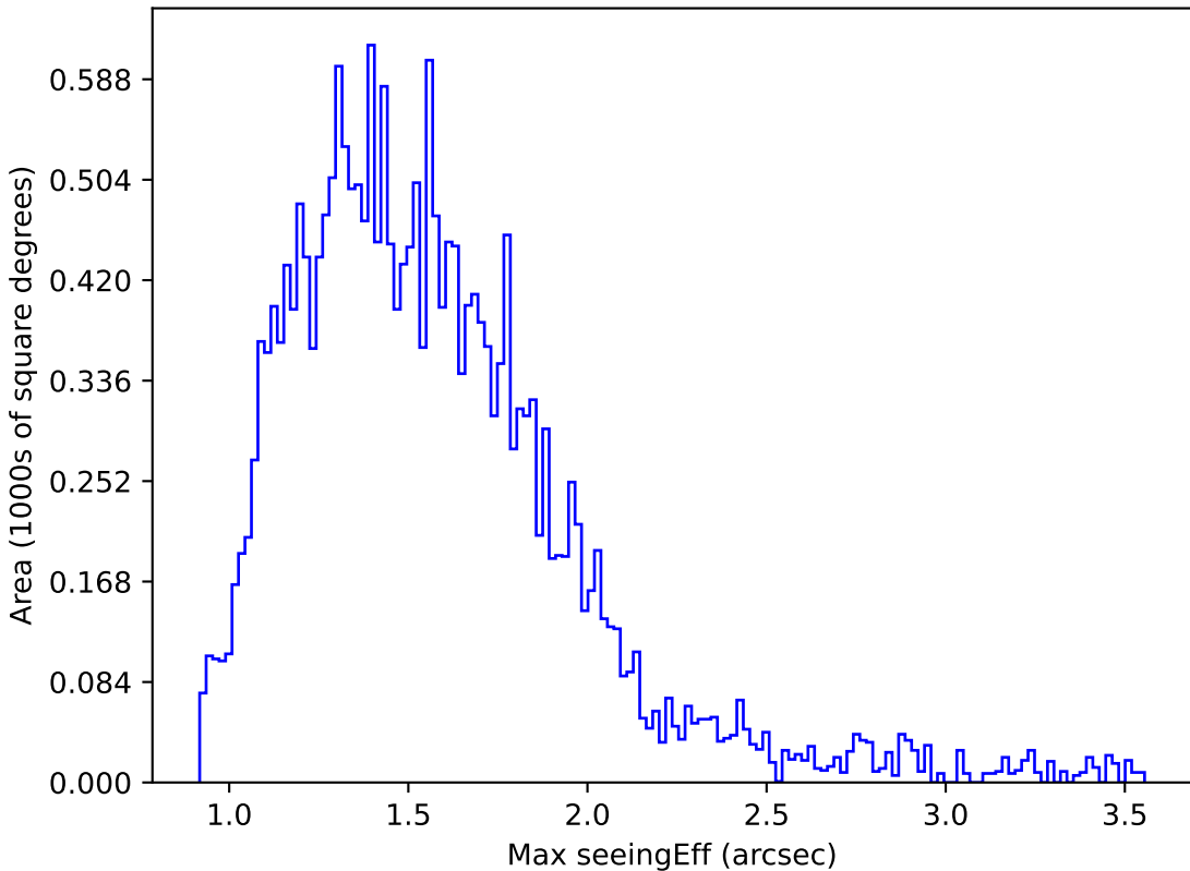
too_elab_r64_d3_giz_v3.4_10yrs Yr 1 u band: Max seeingEff
