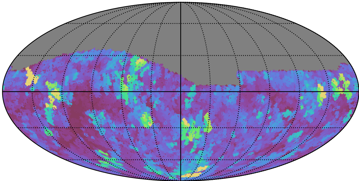
too_elab_r64_d3_giz_v3.4_10yrs Yr 1 i band: Max seeingEff
