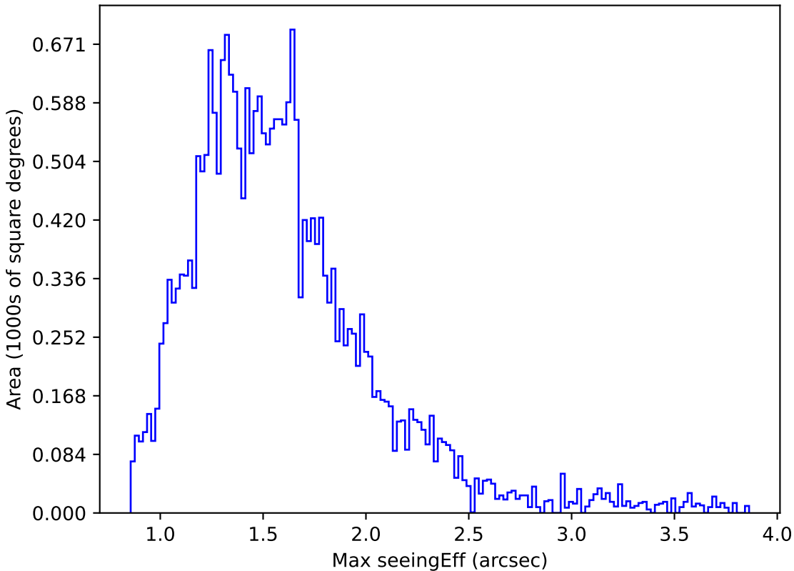
too_elab_r64_d3_giz_v3.4_10yrs Yr 1 g band: Max seeingEff
