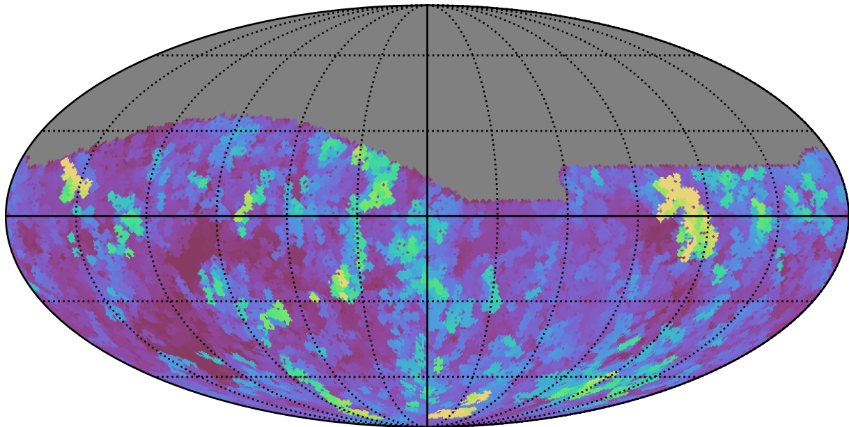
too_elab_r64_d3_giz_v3.4_10yrs Yr 1 all bands: Max seeingEff
