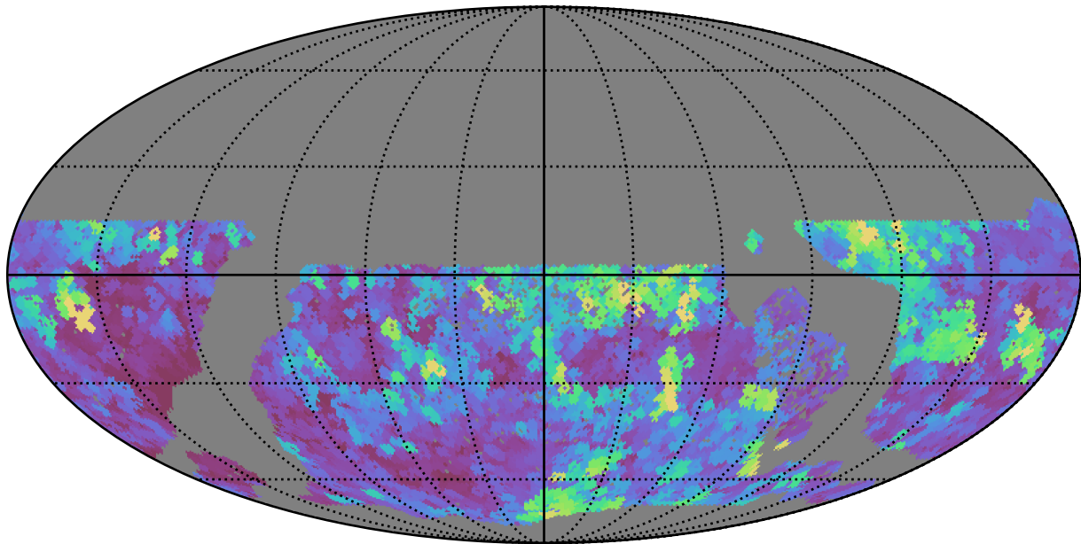
too_elab_r64_d3_giz_v3.4_10yrs WFD all bands: Max seeingEff
