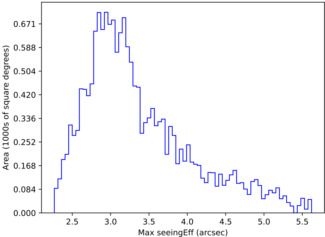
too_elab_r64_d3_giz_v3.4_10yrs WFD all bands: Max seeingEff
