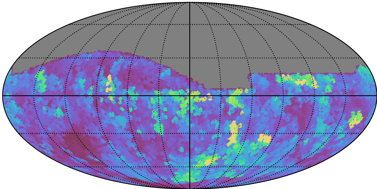
too_elab_r64_d3_giz_v3.4_10yrs All sky z band: Max seeingEff
