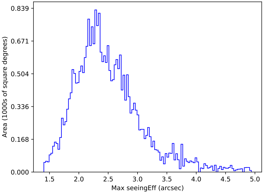
too_elab_r64_d3_giz_v3.4_10yrs All sky z band: Max seeingEff
