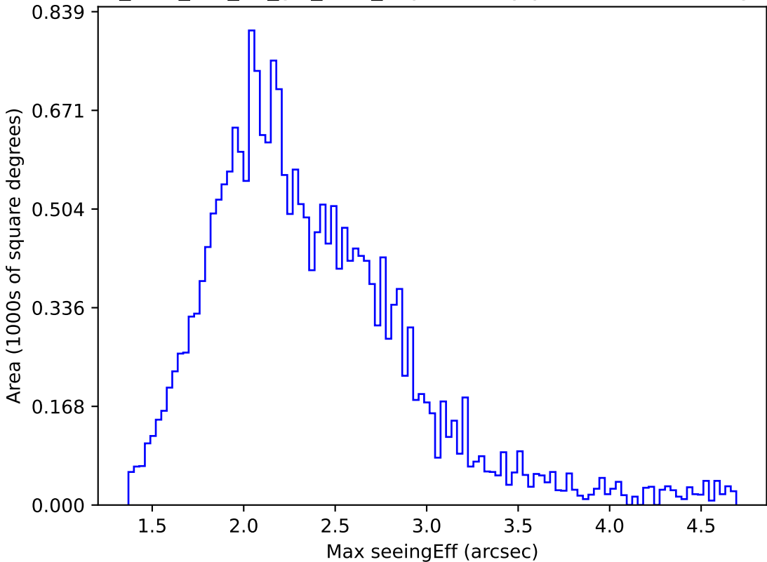
too_elab_r64_d3_giz_v3.4_10yrs All sky y band: Max seeingEff
